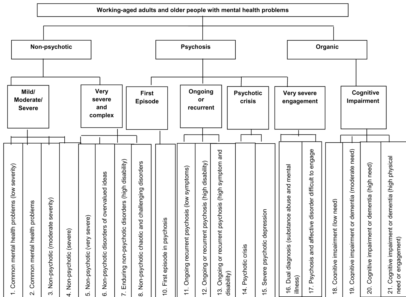
Figure 1. Care Clusters Decision Tree.
